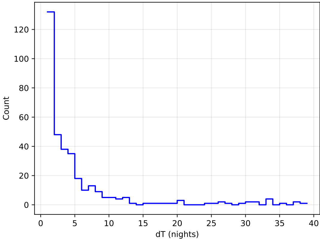
too_ignore_5_1v3.4_10yrs all bands: DD:WFD Delta Nights Histogram
