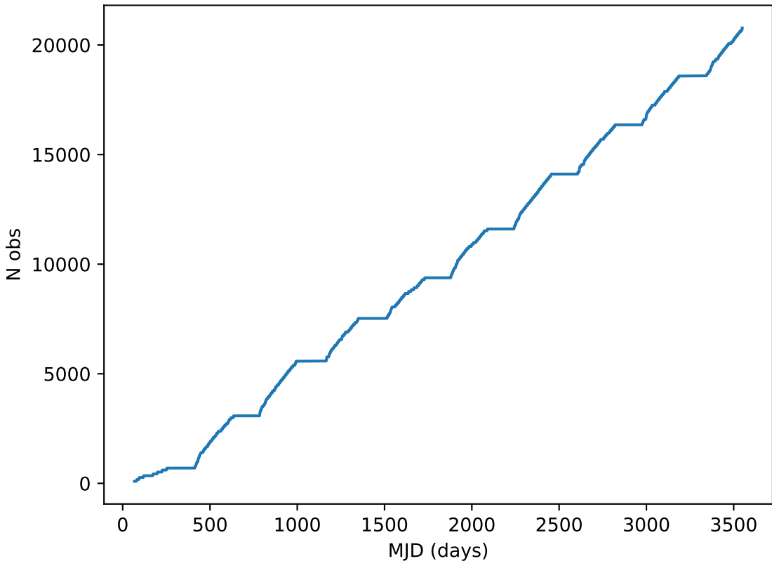
too_ignore_5_1v3.4_10yrs all bands: DD:ELAISS1 Cumulative NVisits
