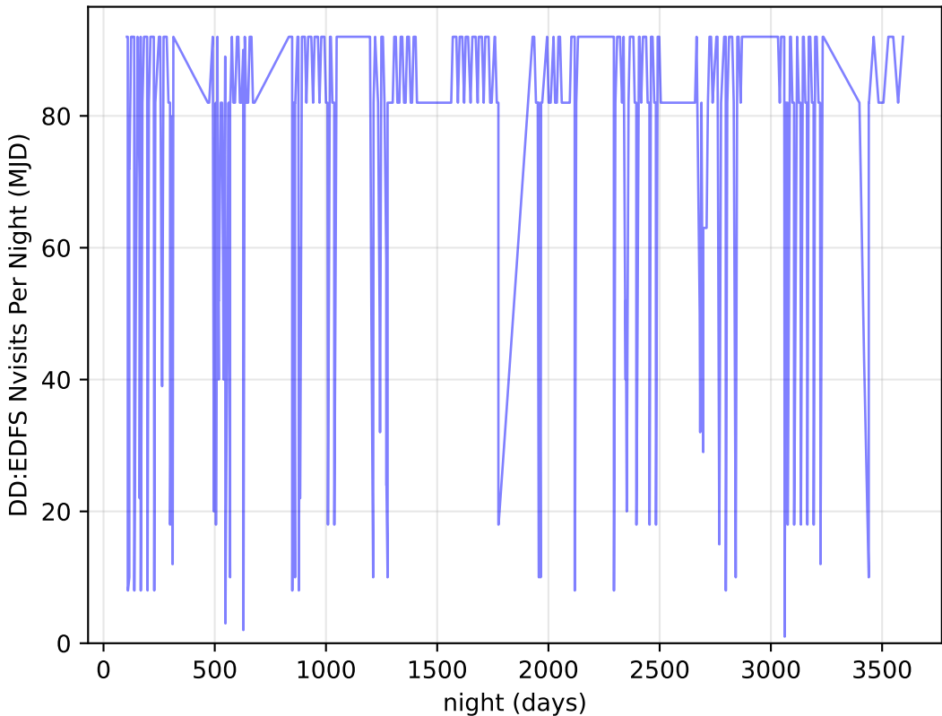
too_ignore_5_1v3.4_10yrs all bands: DD:EDFS Nvisits Per Night
