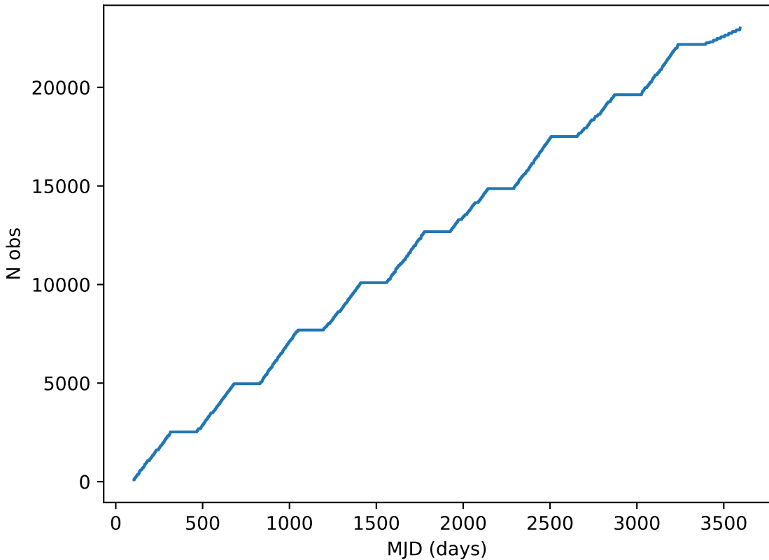
too_ignore_5_1v3.4_10yrs all bands: DD:EDFS Cumulative NVisits
