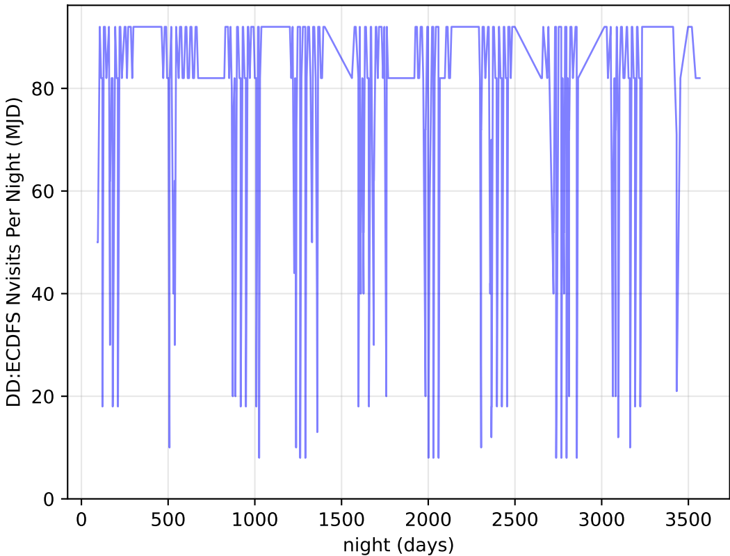
too_ignore_5_1v3.4_10yrs all bands: DD:ECDFS Nvisits Per Night
