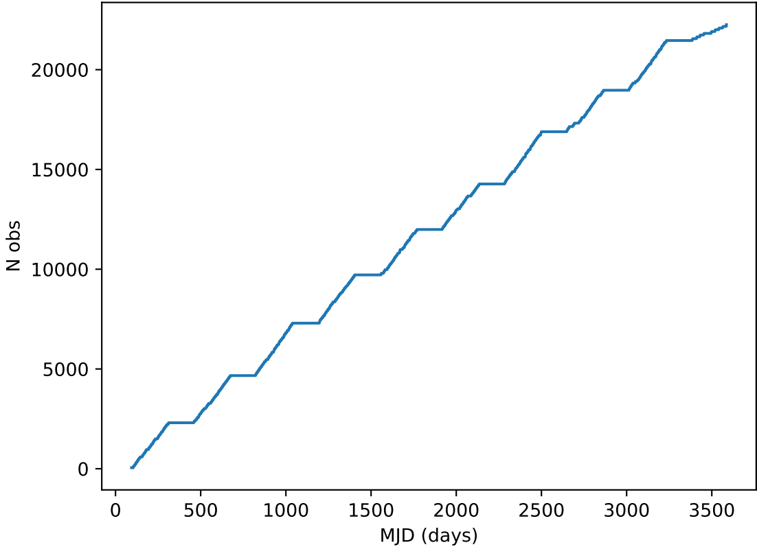
too_ignore_5_1v3.4_10yrs all bands: DD:ECDFS Cumulative NVisits
