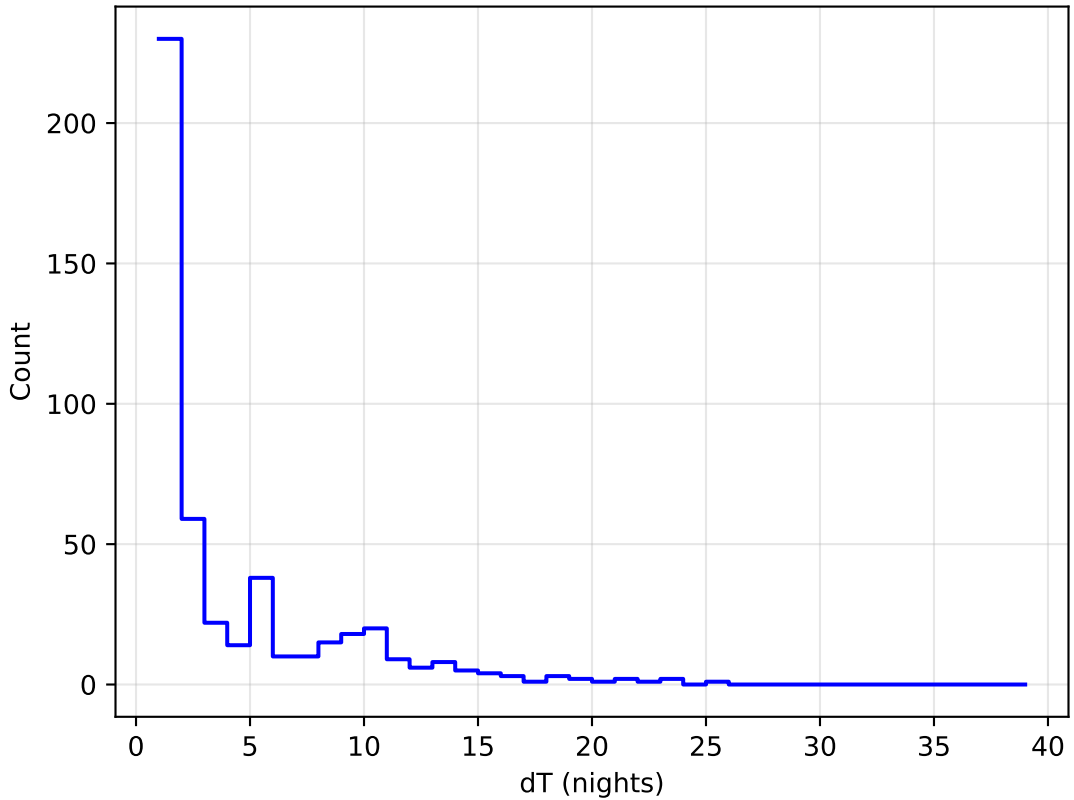
too_ignore_5_1v3.4_10yrs all bands: DD: COSMOS Delta Nights Histogram
