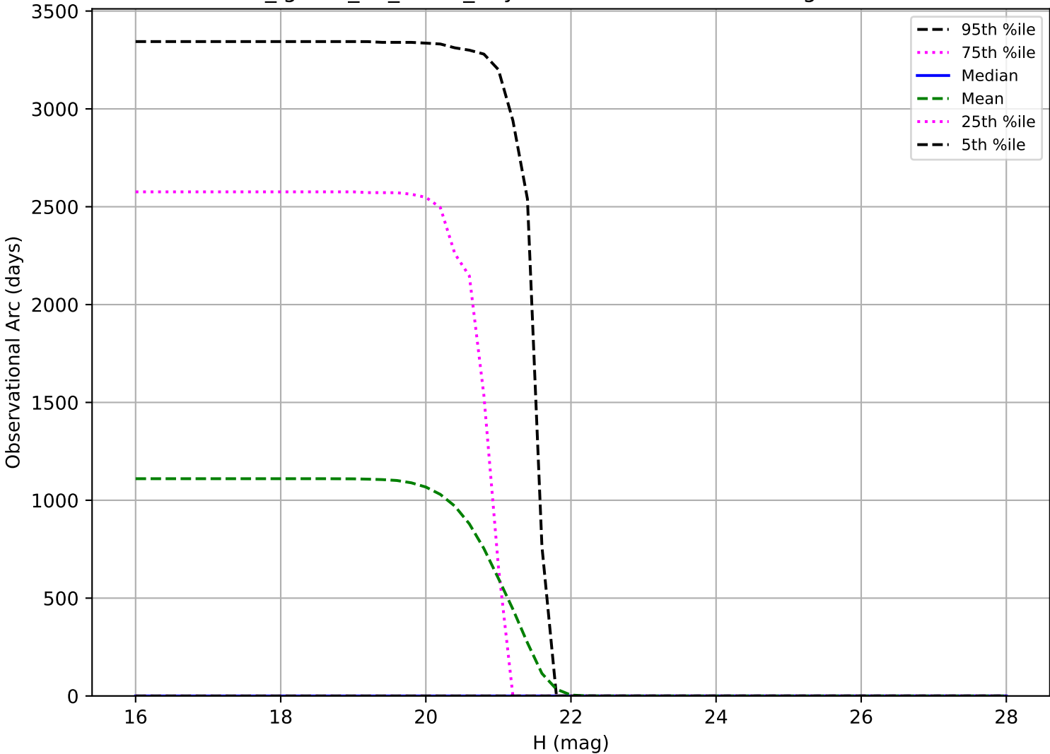
too_ignore_10_4v3.4_10yrs: Observational Arc Length Vatira
