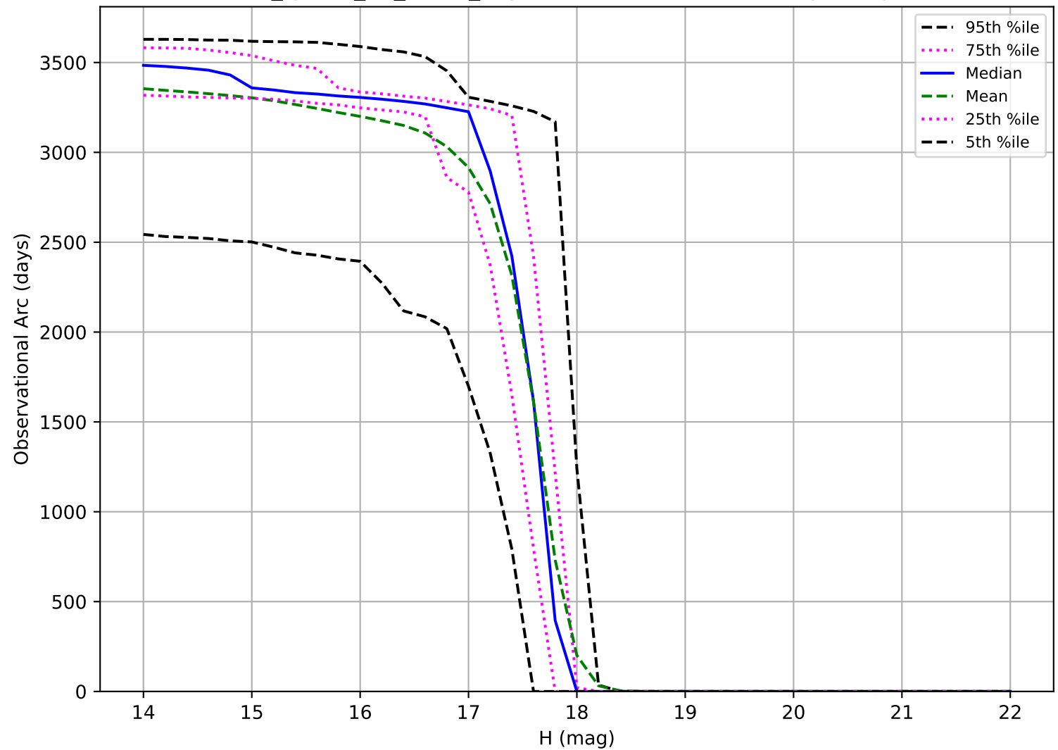
too_ignore_10_4v3.4_10yrs: Observational Arc Length Trojan
