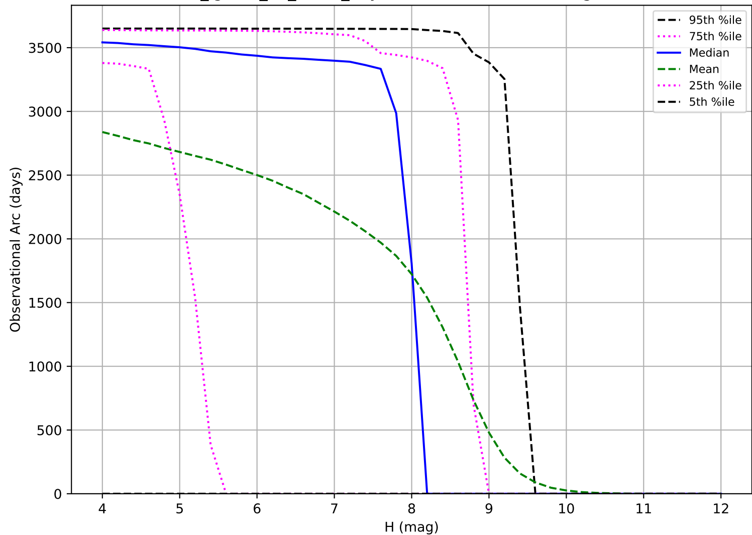
too_ignore_10_4v3.4_10yrs: Observational Arc Length TNO
