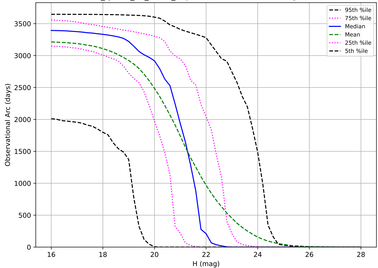
too_ignore_10_4v3.4_10yrs: Observational Arc Length PHA
