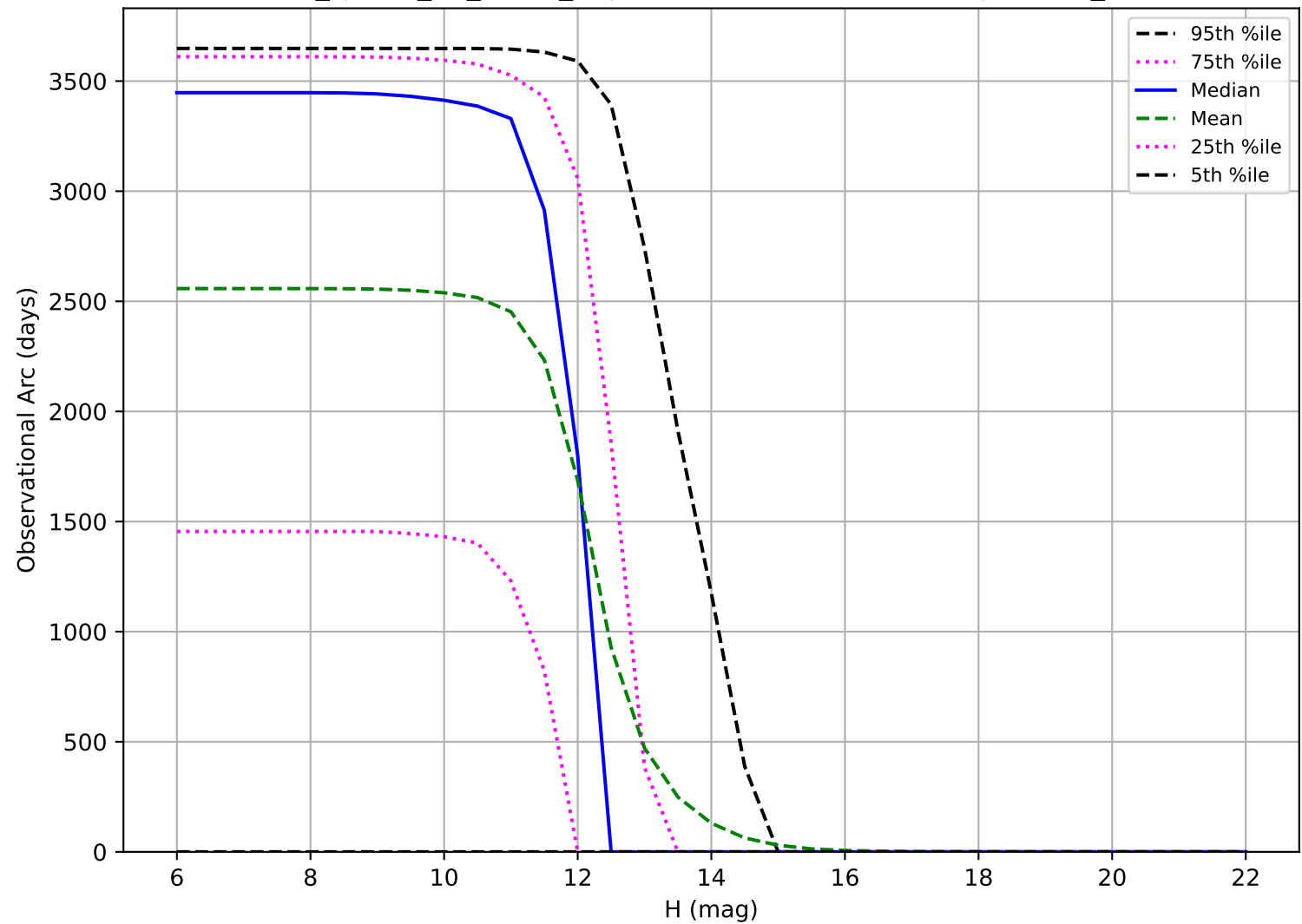
too_ignore_10_4v3.4_10yrs: Observational Arc Length OCC_r20
