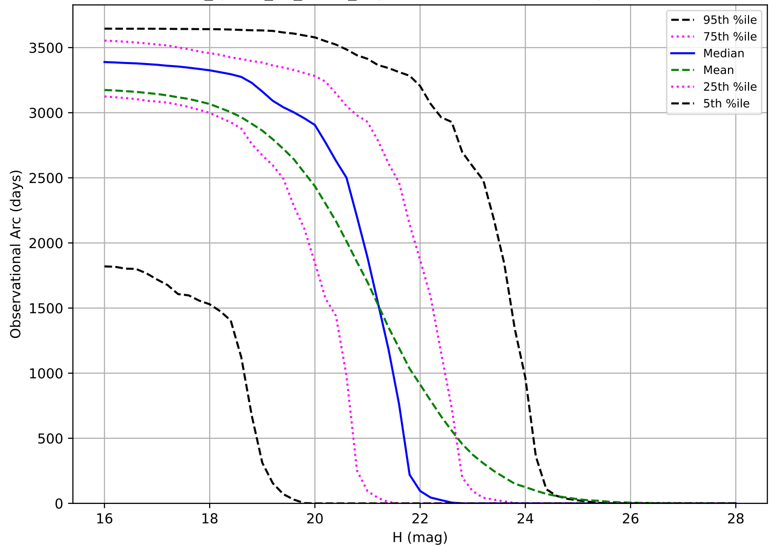
too_ignore_10_4v3.4_10yrs: Observational Arc Length NEO
