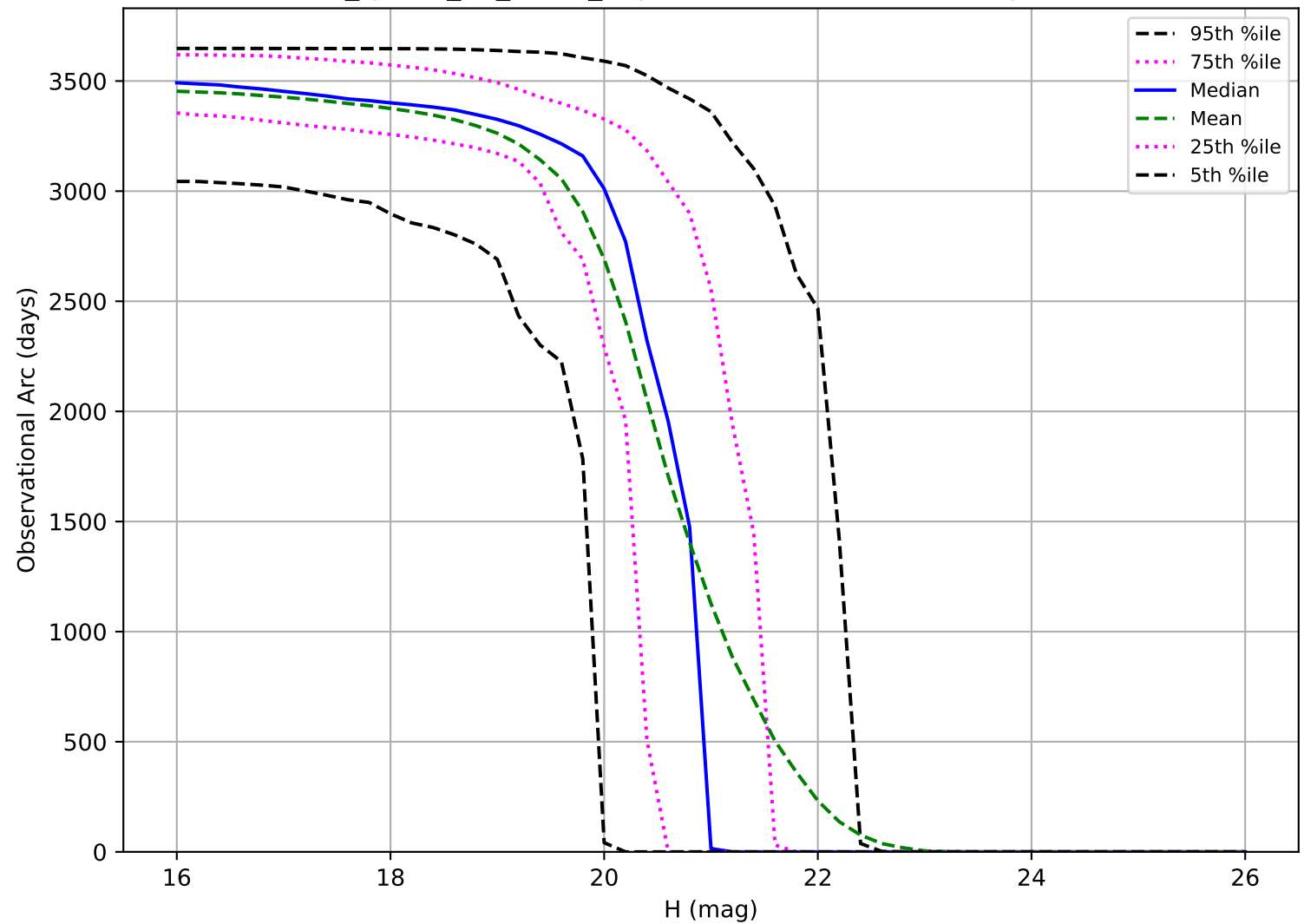
too_ignore_10_4v3.4_10yrs: Observational Arc Length MBA
