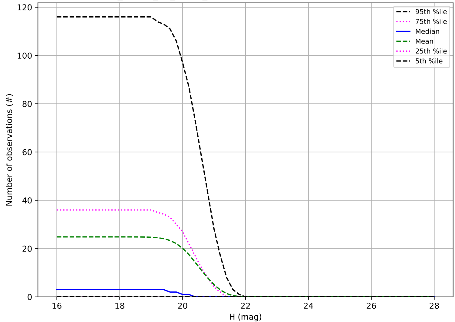
too_ignore_10_4v3.4_10yrs: Number of observations Vatira
