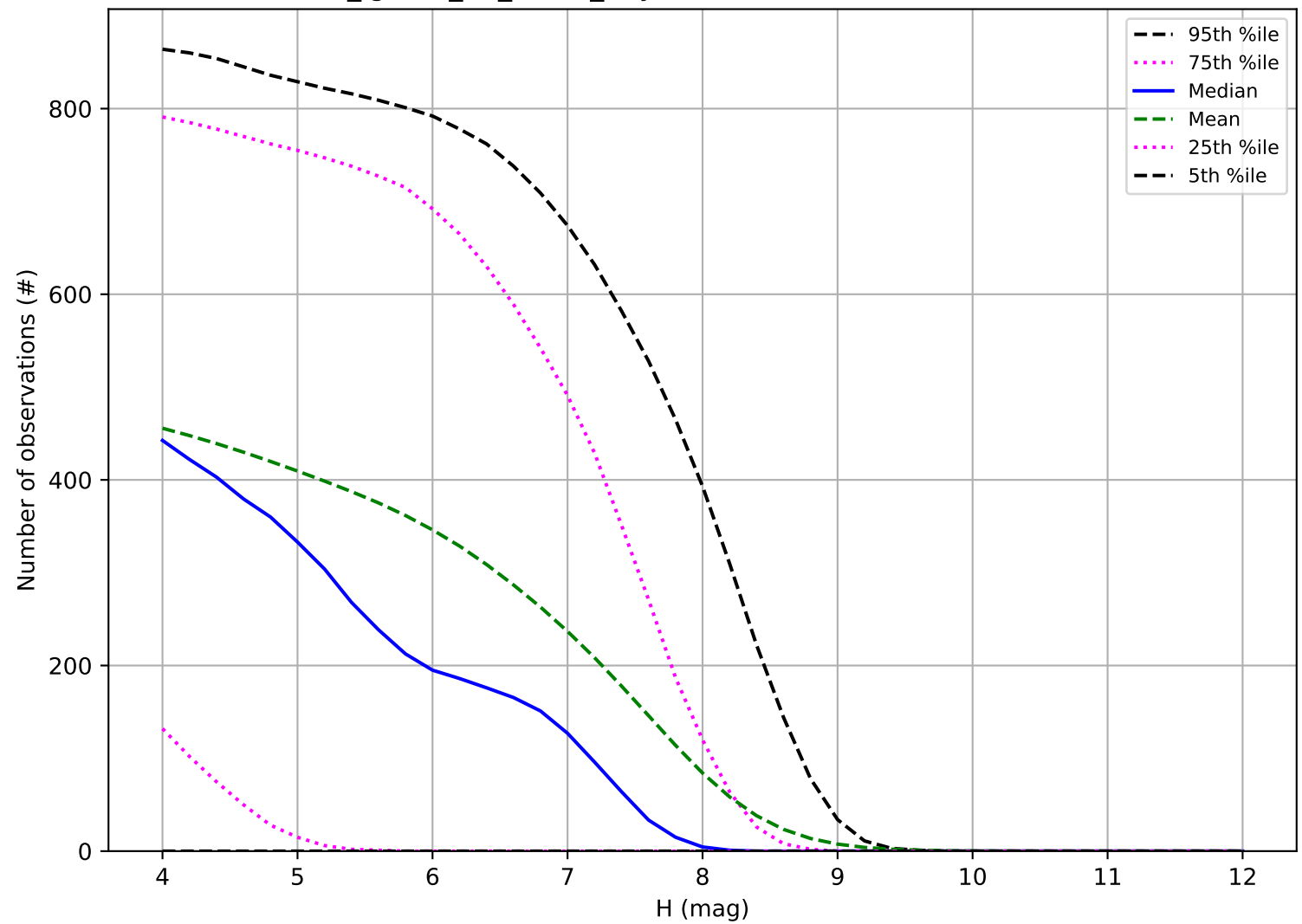
too_ignore_10_4v3.4_10yrs: Number of observations TNO
