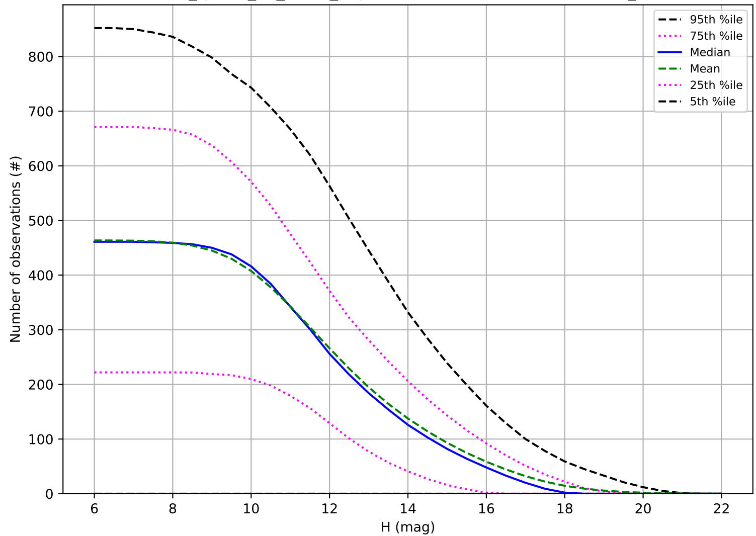
too_ignore_10_4v3.4_10yrs: Number of observations OCC_r5
