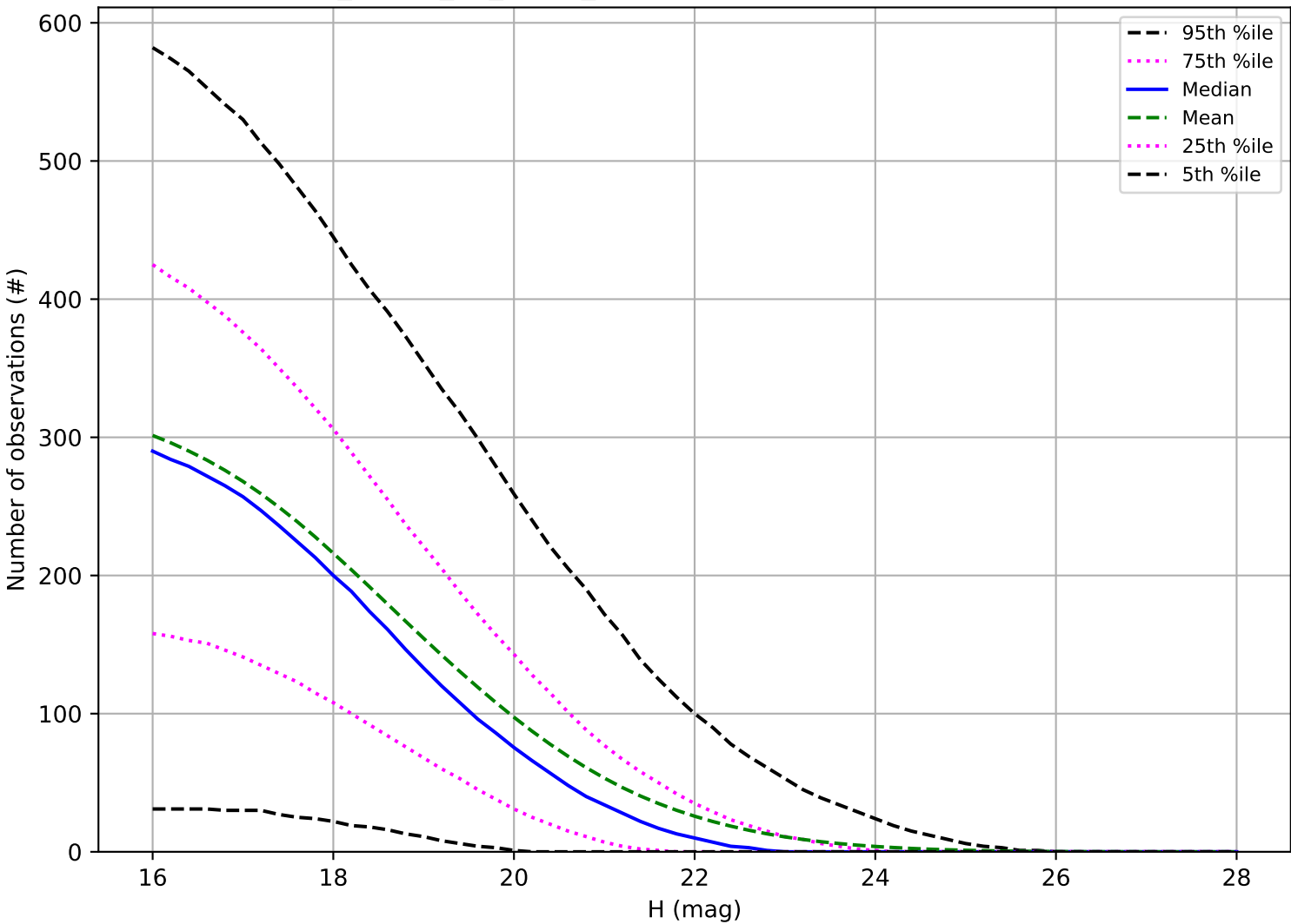
too_ignore_10_4v3.4_10yrs: Number of observations NEO
