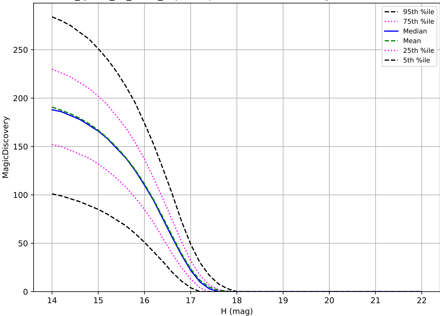
too_ignore_10_4v3.4_10yrs: Trojan 6 detections in 60 nights detection loss
