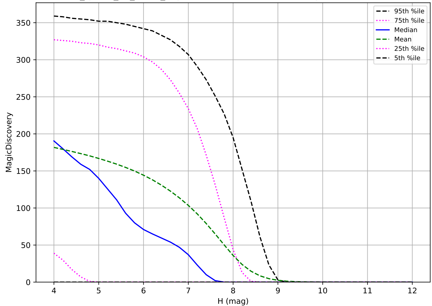
too_ignore_10_4v3.4_10yrs: TNO 6 detections in 60 nights detection loss
