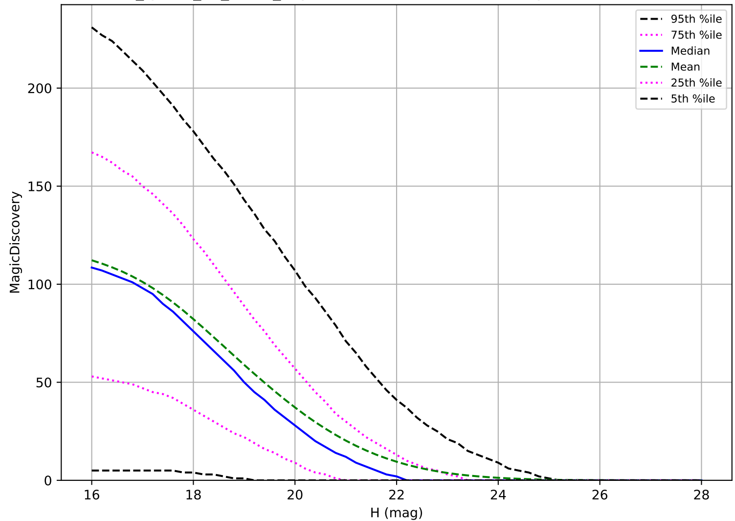
too_ignore_10_4v3.4_10yrs: NEO 6 detections in 60 nights detection loss
