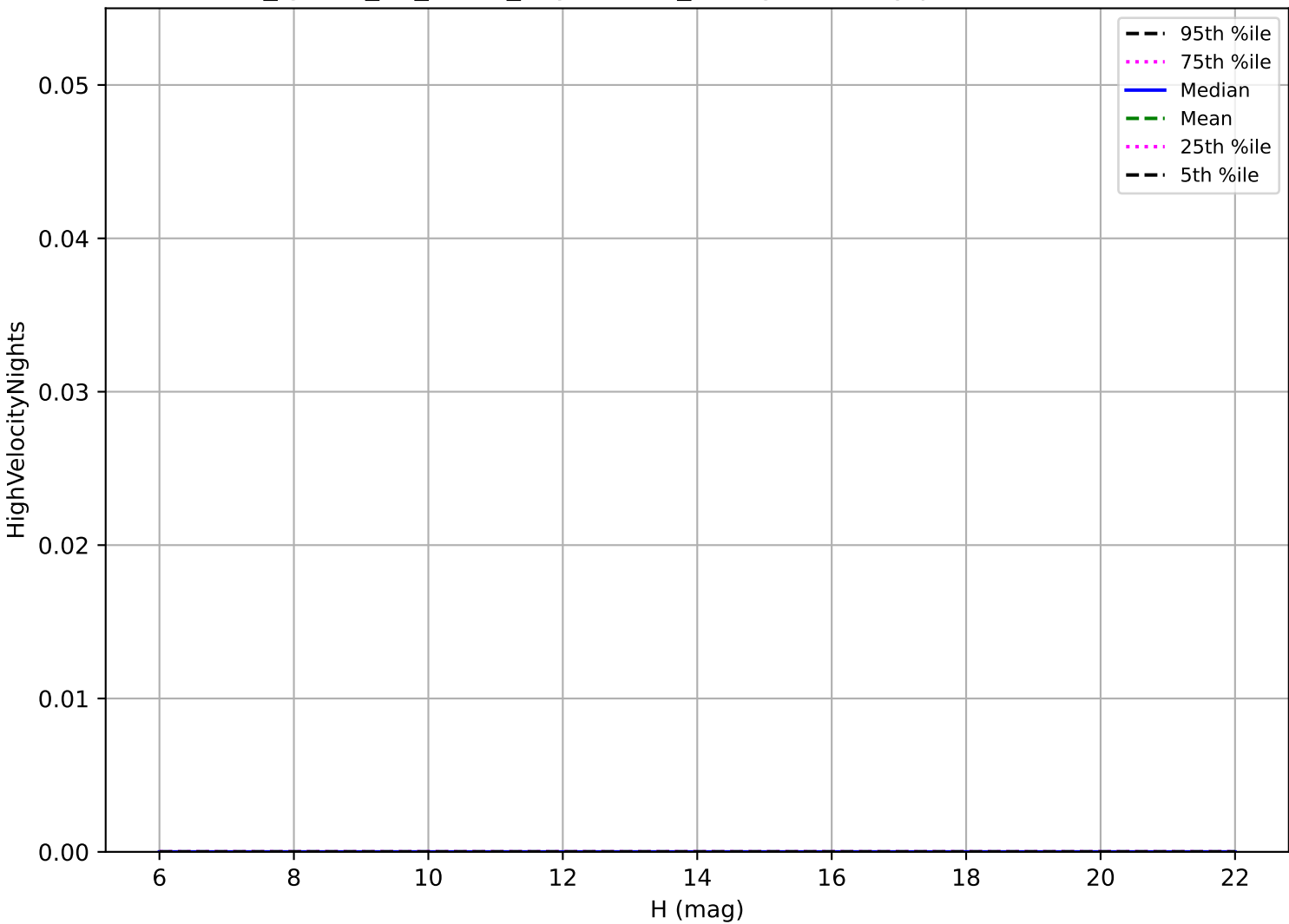
too_ignore_10_4v3.4_10yrs: OCC_r5 High velocity pair detection loss
