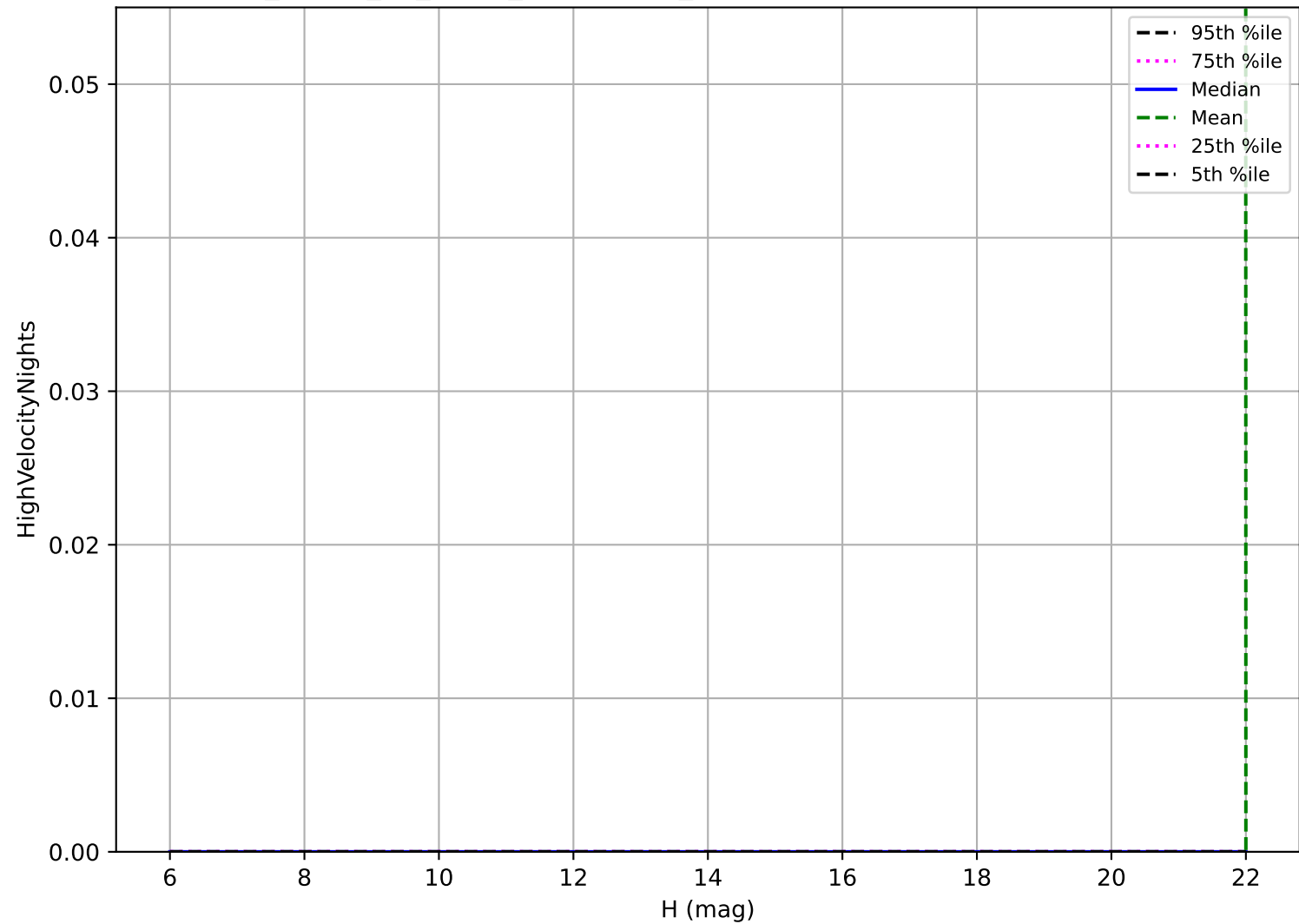
too_ignore_10_4v3.4_10yrs: OCC_r20 High velocity pair detection loss
