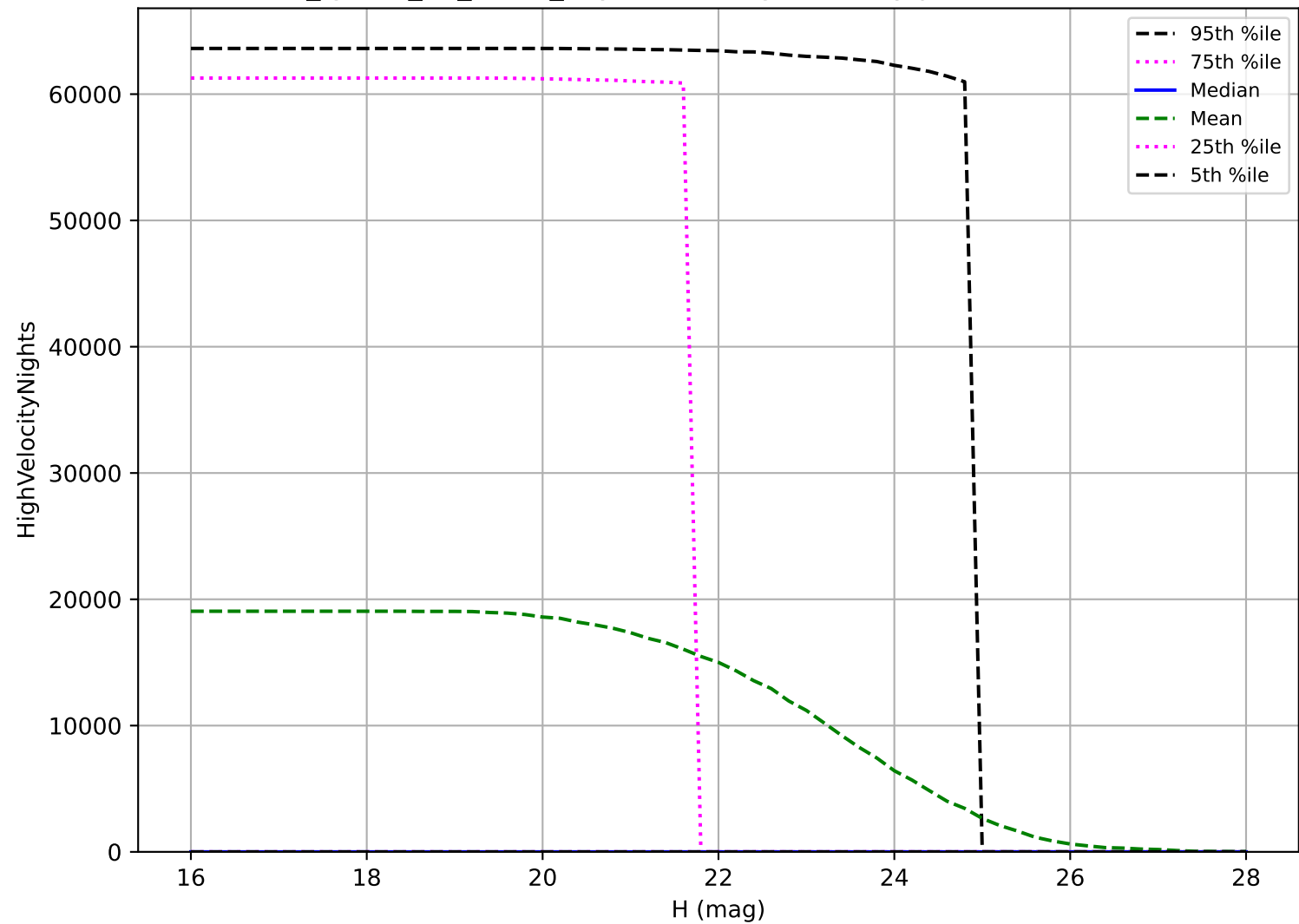
too_ignore_10_4v3.4_10yrs: NEO High velocity pair detection loss
