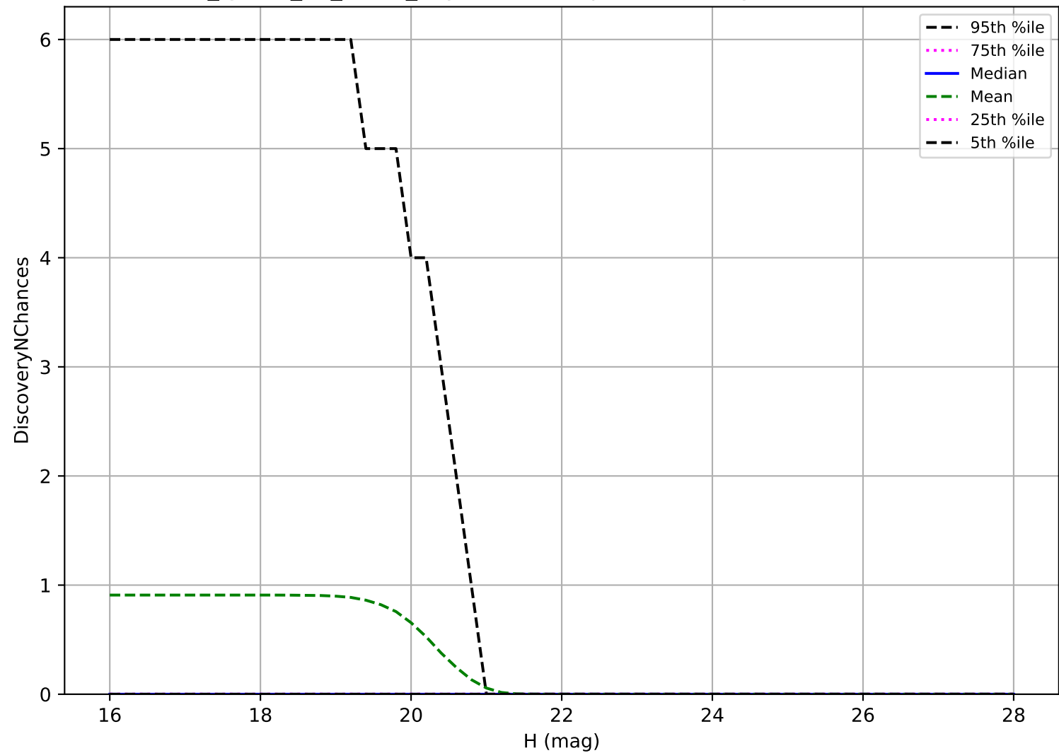
too_ignore_10_4v3.4_10yrs: Vatira 3 pairs in 15 nights detection loss
