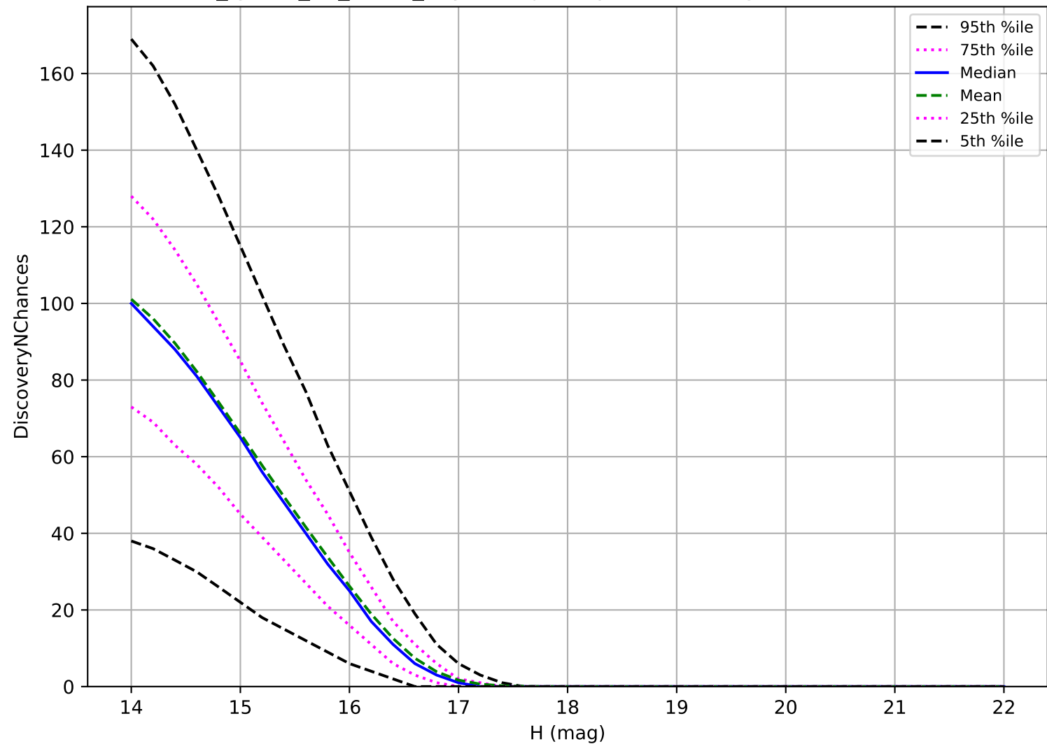
too_ignore_10_4v3.4_10yrs: Trojan 3 pairs in 15 nights detection loss
