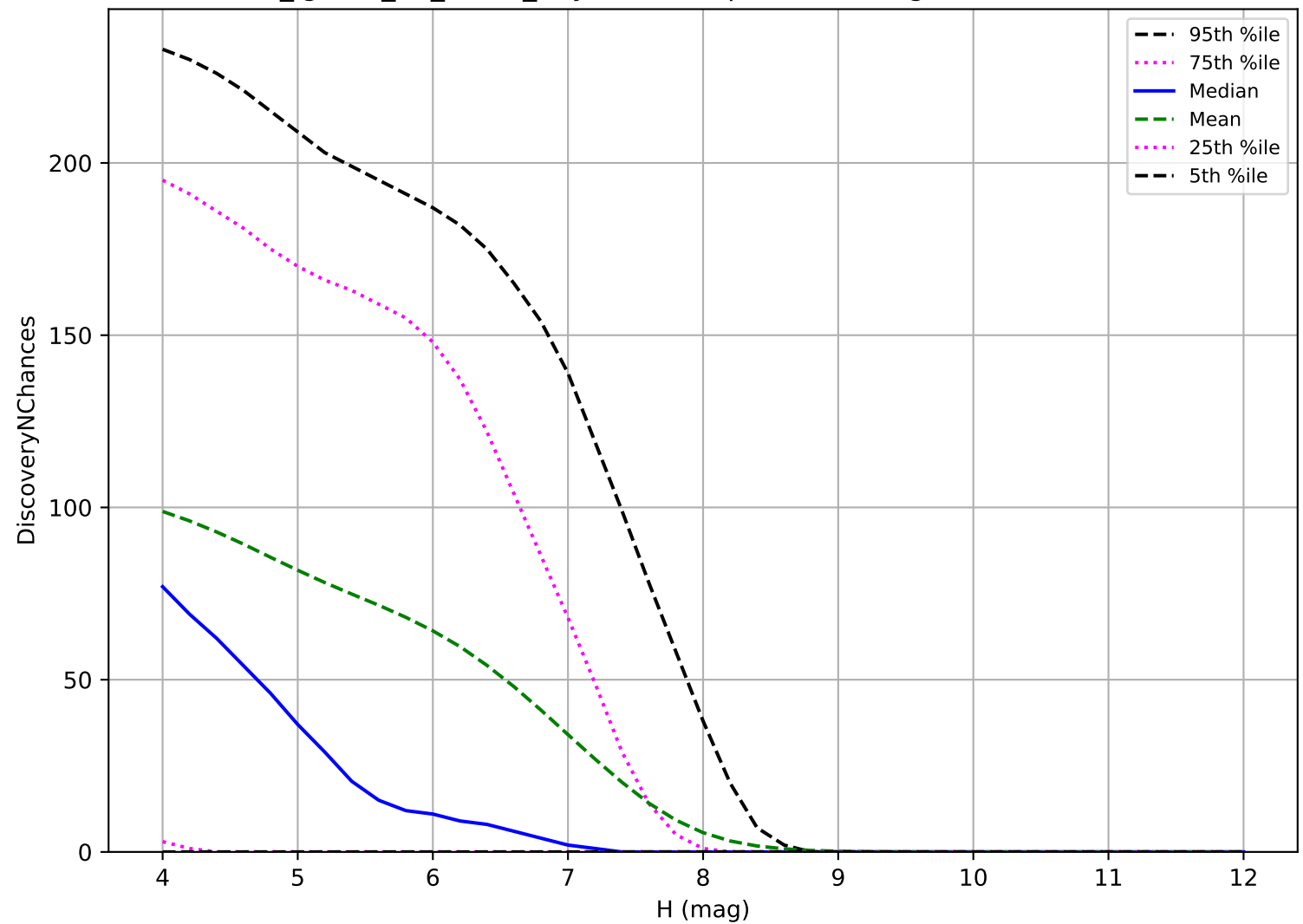
too_ignore_10_4v3.4_10yrs: TNO 3 pairs in 15 nights detection loss
