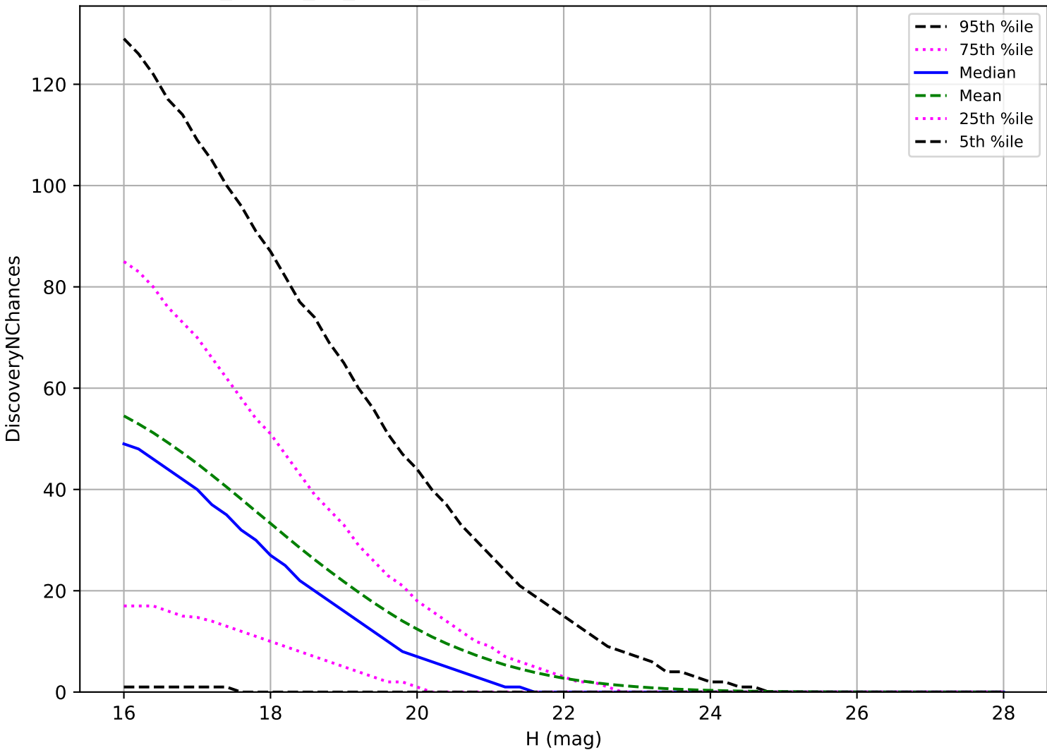
too_ignore_10_4v3.4_10yrs: PHA 3 pairs in 15 nights detection loss
