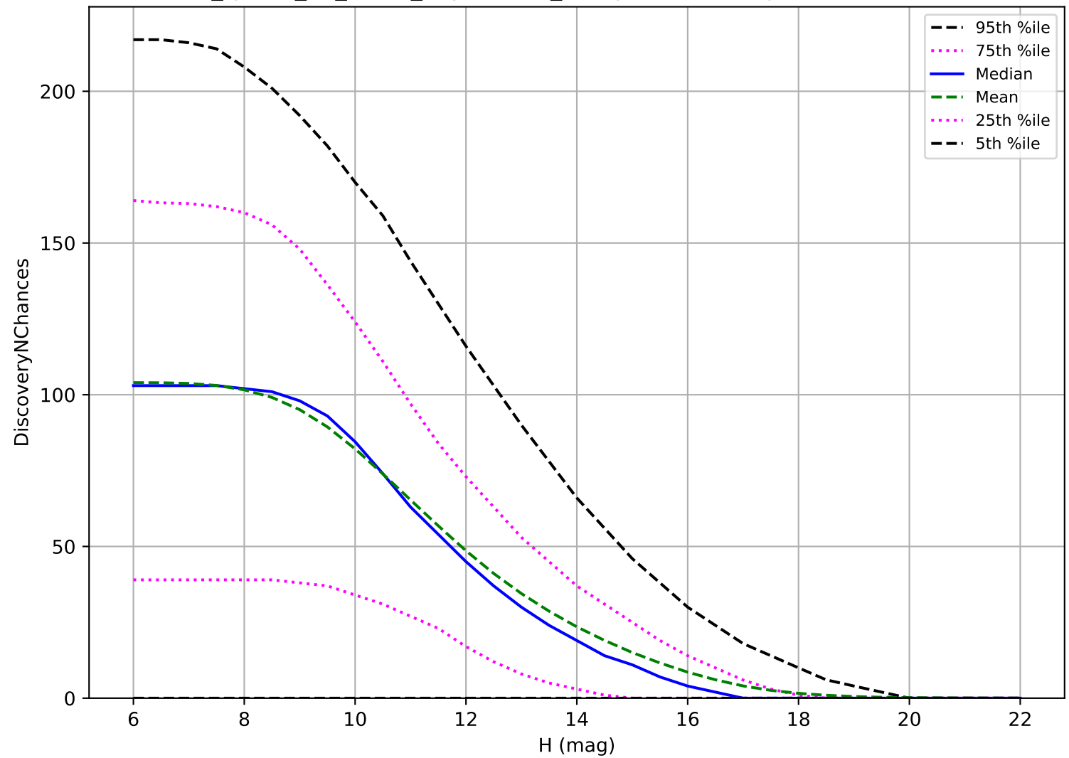
too_ignore_10_4v3.4_10yrs: OCC_r5 3 pairs in 15 nights detection loss
