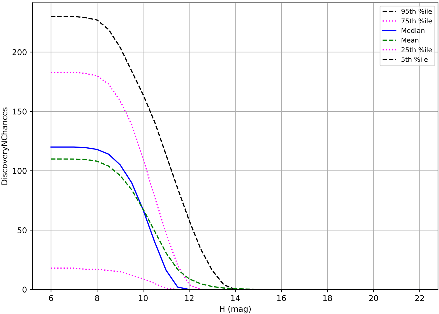
too_ignore_10_4v3.4_10yrs: OCC_r20 3 pairs in 15 nights detection loss
