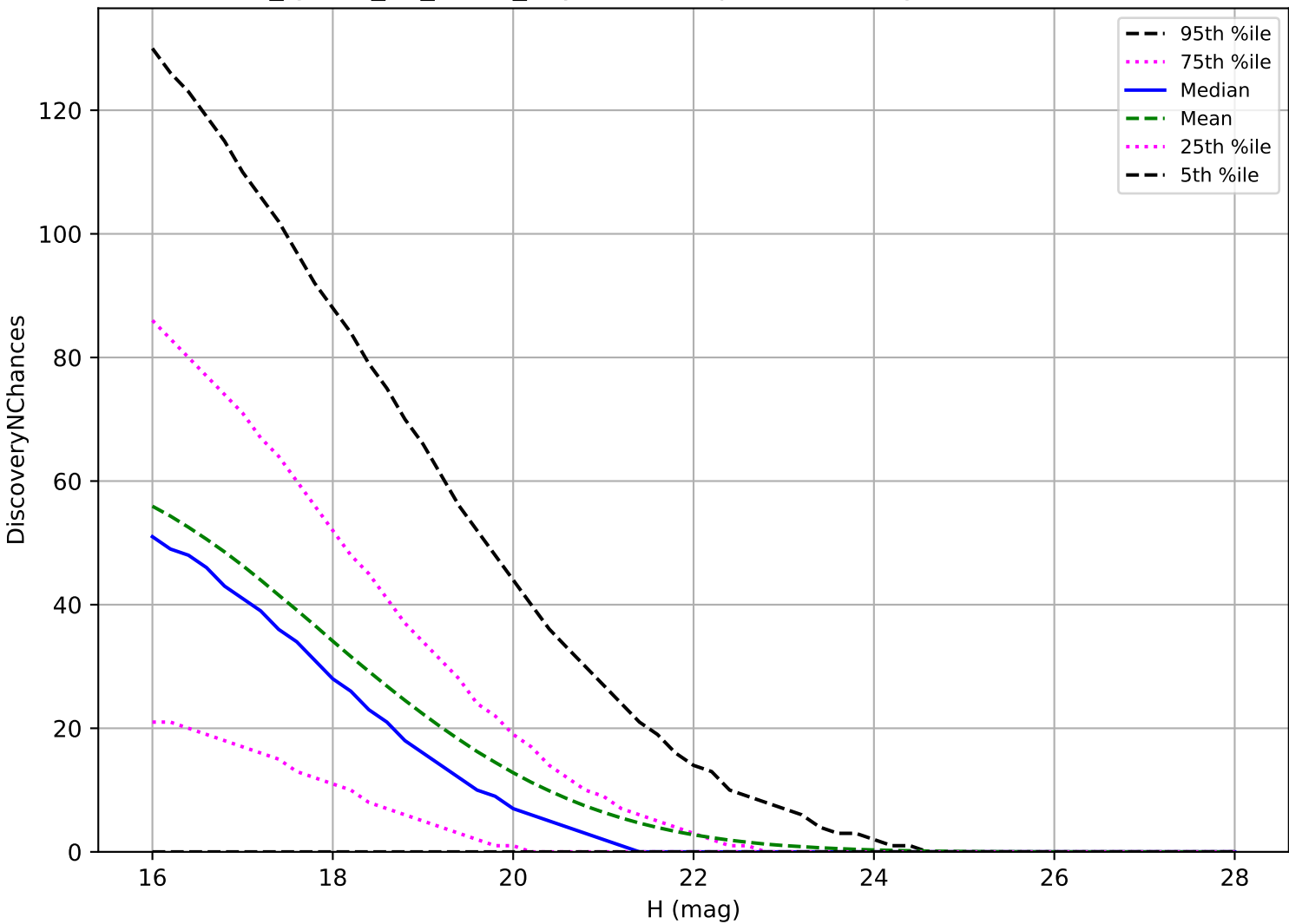
too_ignore_10_4v3.4_10yrs: NEO 3 pairs in 15 nights detection loss
