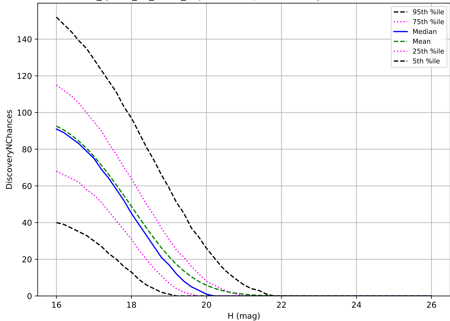
too_ignore_10_4v3.4_10yrs: MBA 3 pairs in 15 nights detection loss
