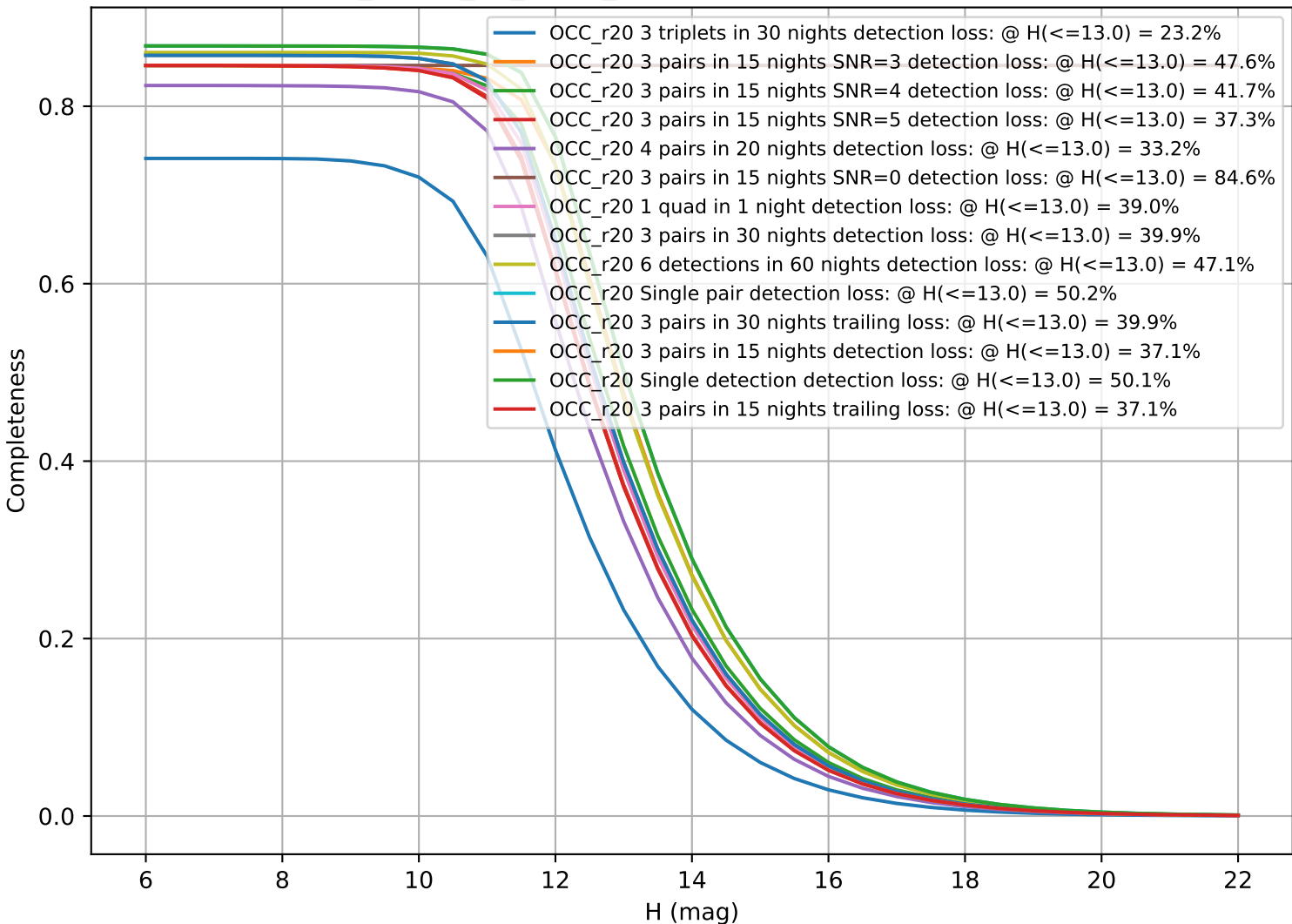
too_ignore_10_4v3.4_10yrs: CumulativeCompleteness
