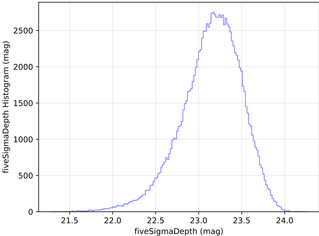
too_ignore_10_4v3.4_10yrs u: fiveSigmaDepth Histogram
