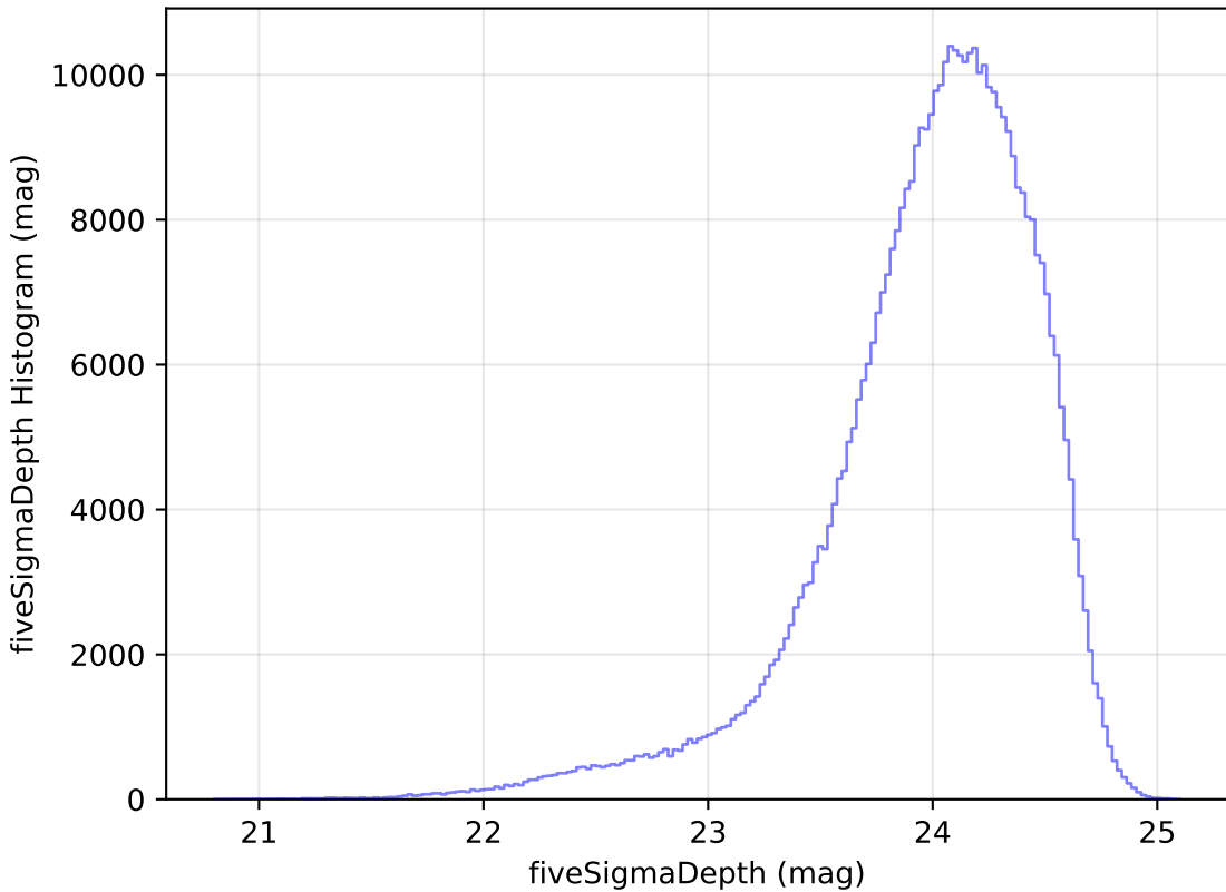
too_ignore_10_4v3.4_10yrs r: fiveSigmaDepth Histogram
