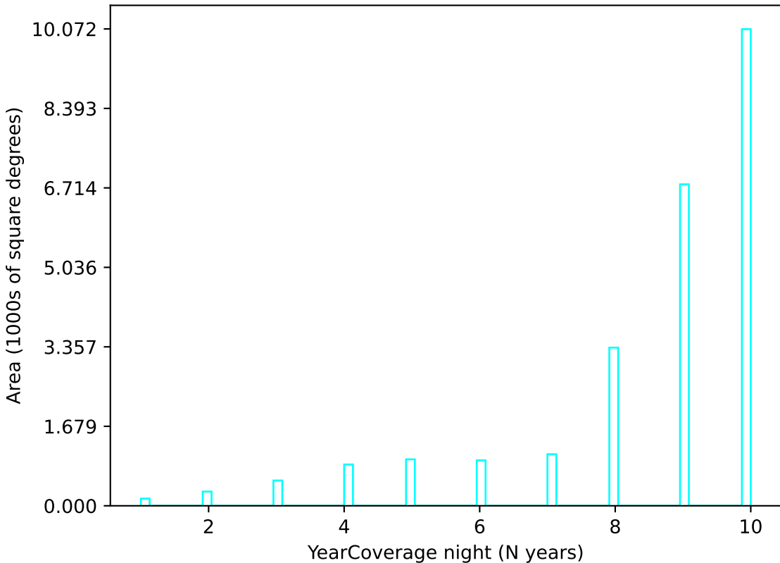
too_ignore_10_4v3.4_10yrs u band: YearCoverage night
