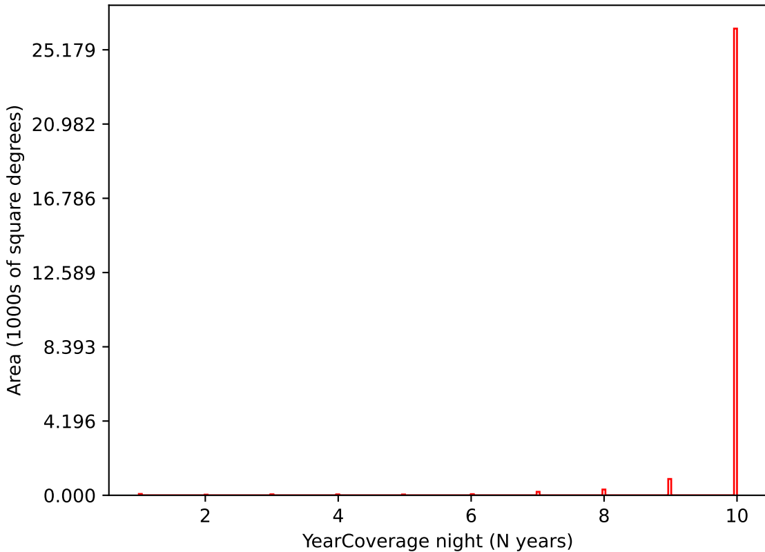
too_ignore_10_4v3.4_10yrs i band: YearCoverage night
