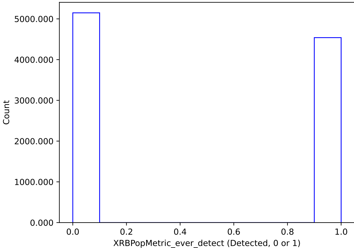
too_ignore_10_4v3.4_10yrs : XRBPoMetric_ever_detect
