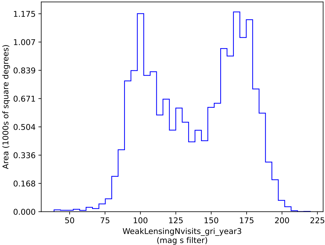
too_ignore_10_4v3.4_10yrs gri band non-DD: WeakLensingNvisits_gri_year3
