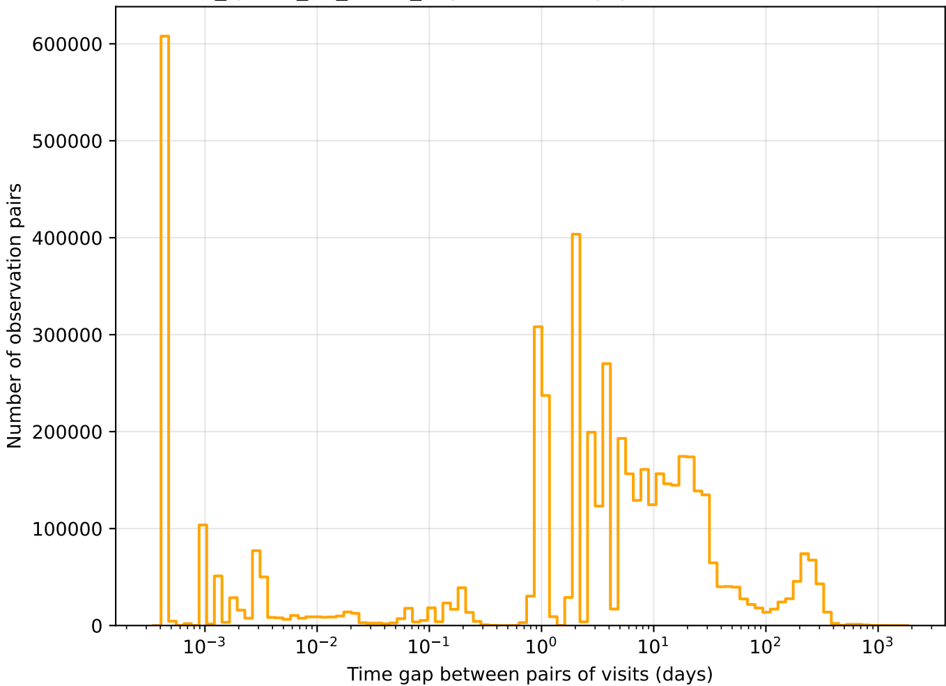
too_ignore_10_4v3.4_10yrs r band: Tgaps observationStartMJD
