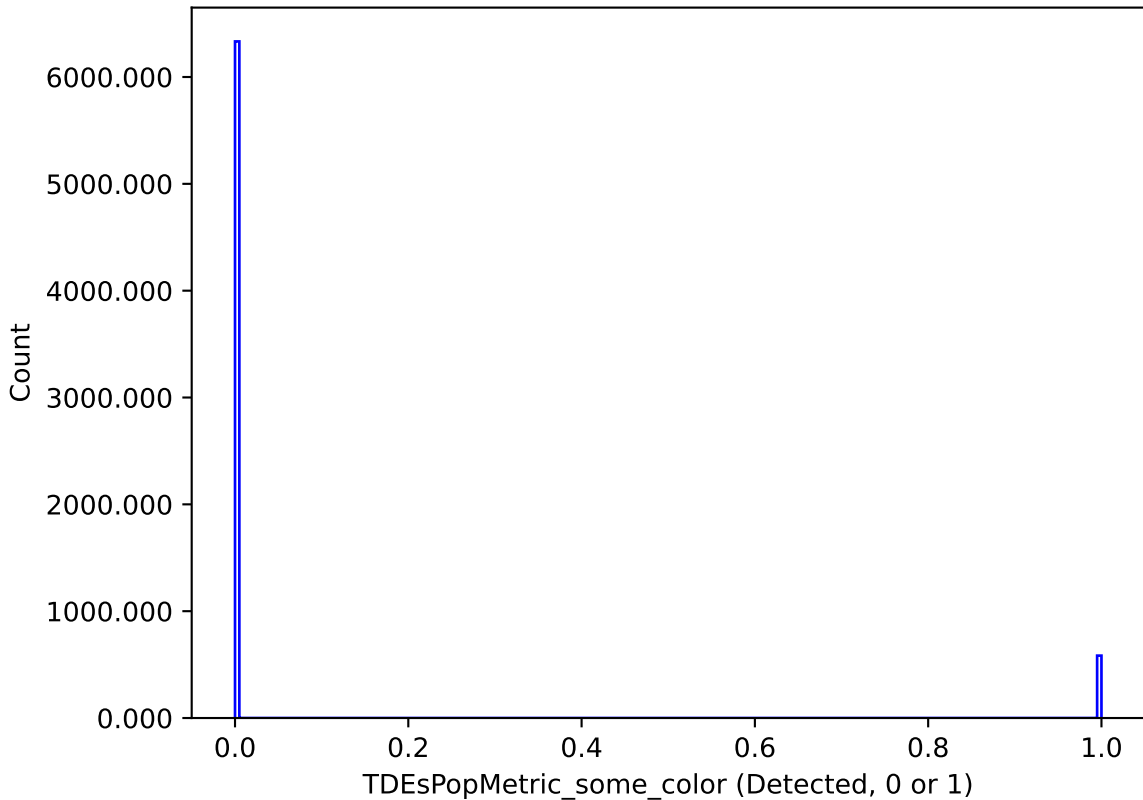
too_ignore_10_4v3.4_10yrs : TDEsPopMetric_some_color
