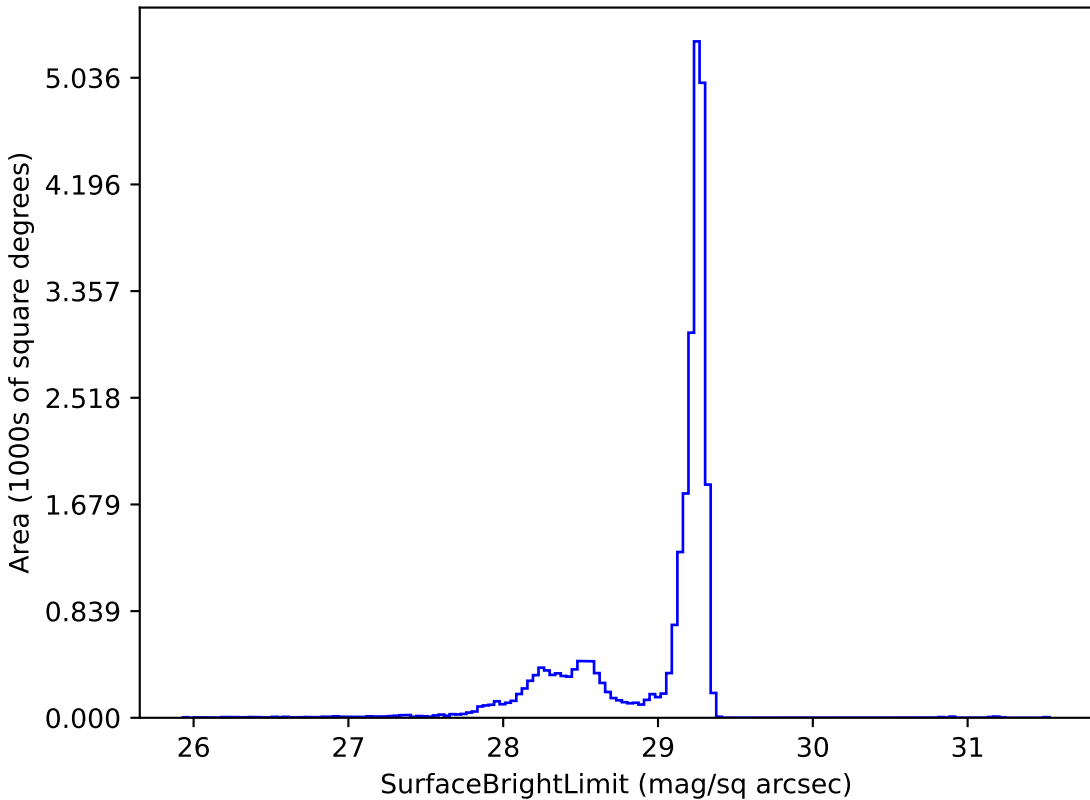
too_ignore_10_4v3.4_10yrs z: SurfaceBrightLimit
