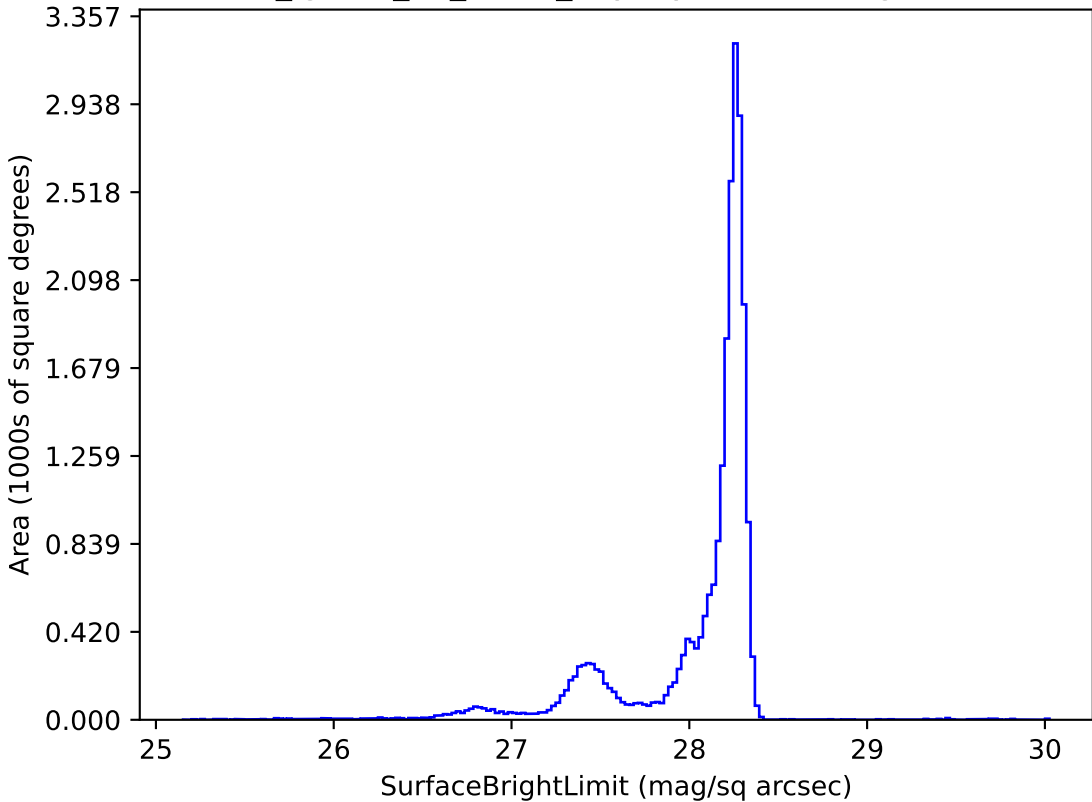
too_ignore_10_4v3.4_10yrs y: SurfaceBrightLimit
