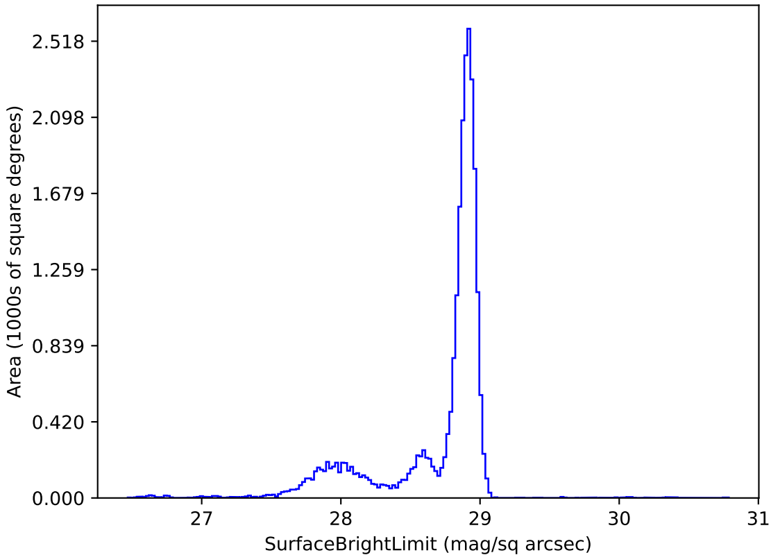
too_ignore_10_4v3.4_10yrs u: SurfaceBrightLimit
