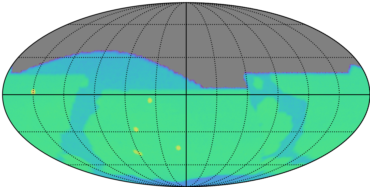
too_ignore_10_4v3.4_10yrs r: SurfaceBrightLimit
