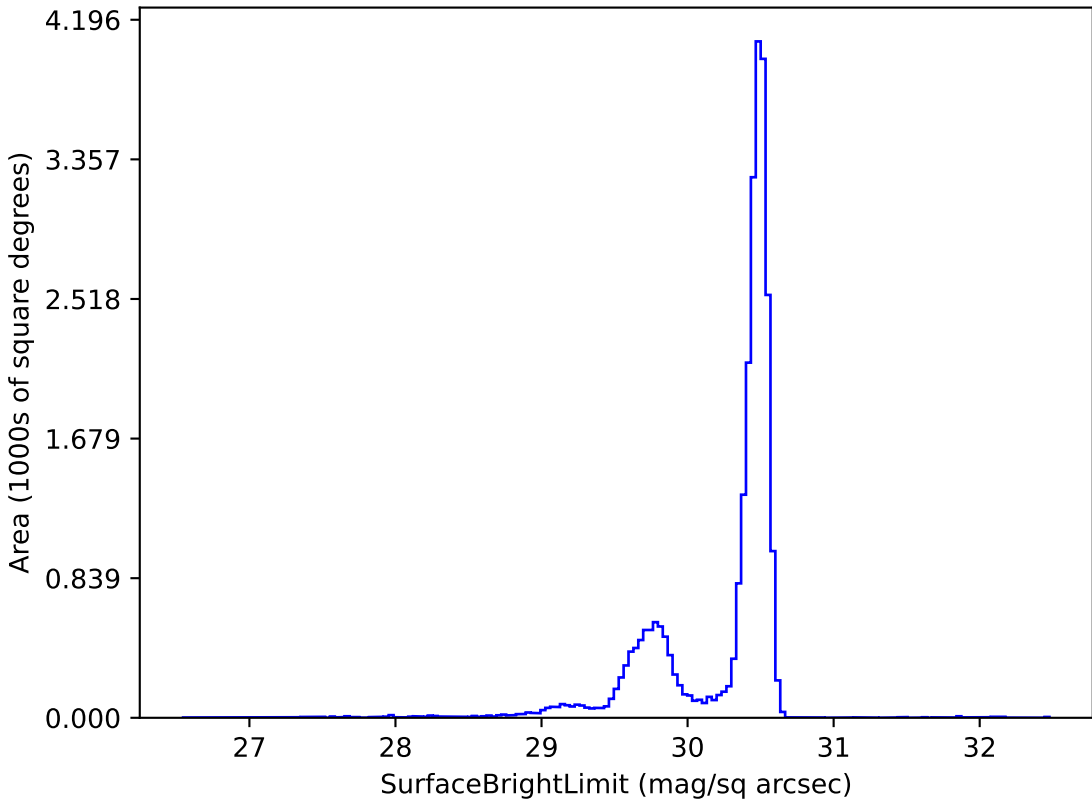
too_ignore_10_4v3.4_10yrs r: SurfaceBrightLimit
