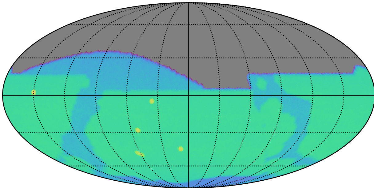
too_ignore_10_4v3.4_10yrs i: SurfaceBrightLimit
