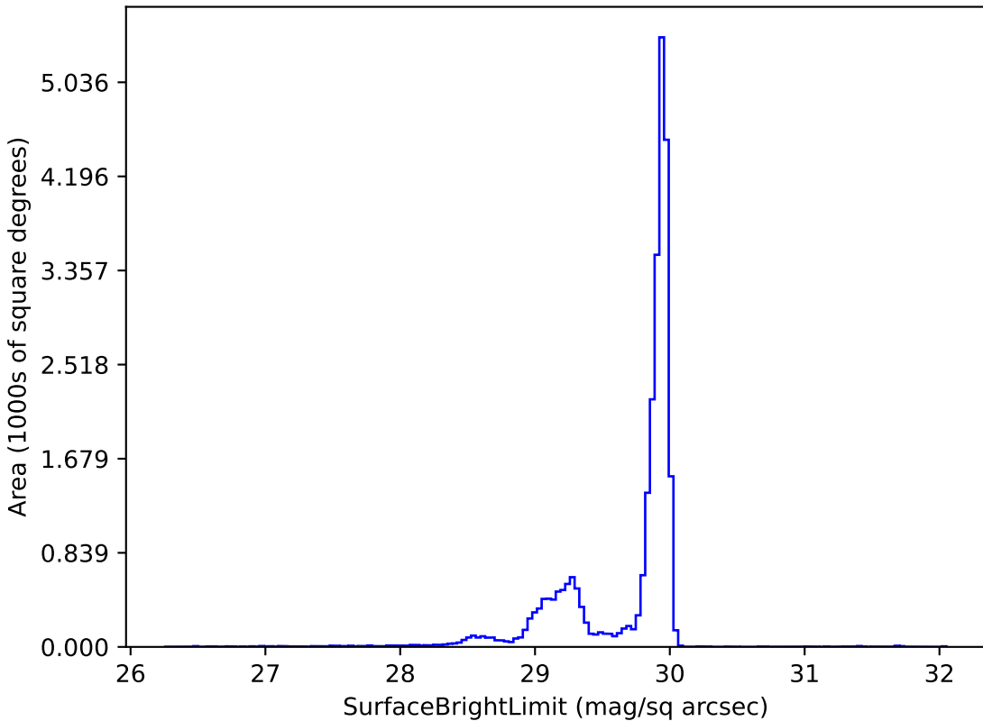
too_ignore_10_4v3.4_10yrs i: SurfaceBrightLimit
