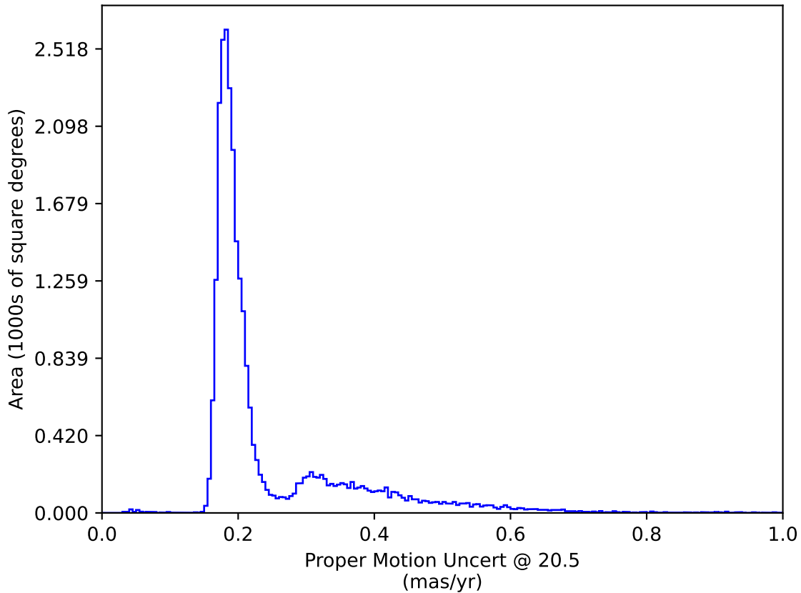
too_ignore_10_4v3.4_10yrs : Proper Motion Uncert @ 20.5
