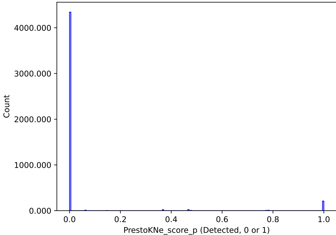
too_ignore_10_4v3.4_10yrs : PrestoKNe_score_p
